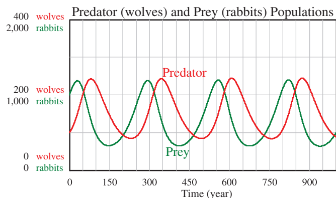
Fig. 1. A typical solution of the predator–prey system obtained by running the system with the following parameter values and initial conditions: a = 3.0 \times 10^{-5} (rabbits·years) ^{-1} ; b = 2.0 \times 10^{-2} years ^{-1} , c = 3.0 \times 10^{-2} years ^{-1} , d = 2.0 \times 10^{-4} (wolves·years) ^{-1} ; x(0) = 1.0 \times 10^{+2} wolves; and y(0) = 1.0 \times 10^{+3} rabbits. Predator population is measured in units of wolves, Prey population is measured in units of rabbits, and Time is measured in units of years.
